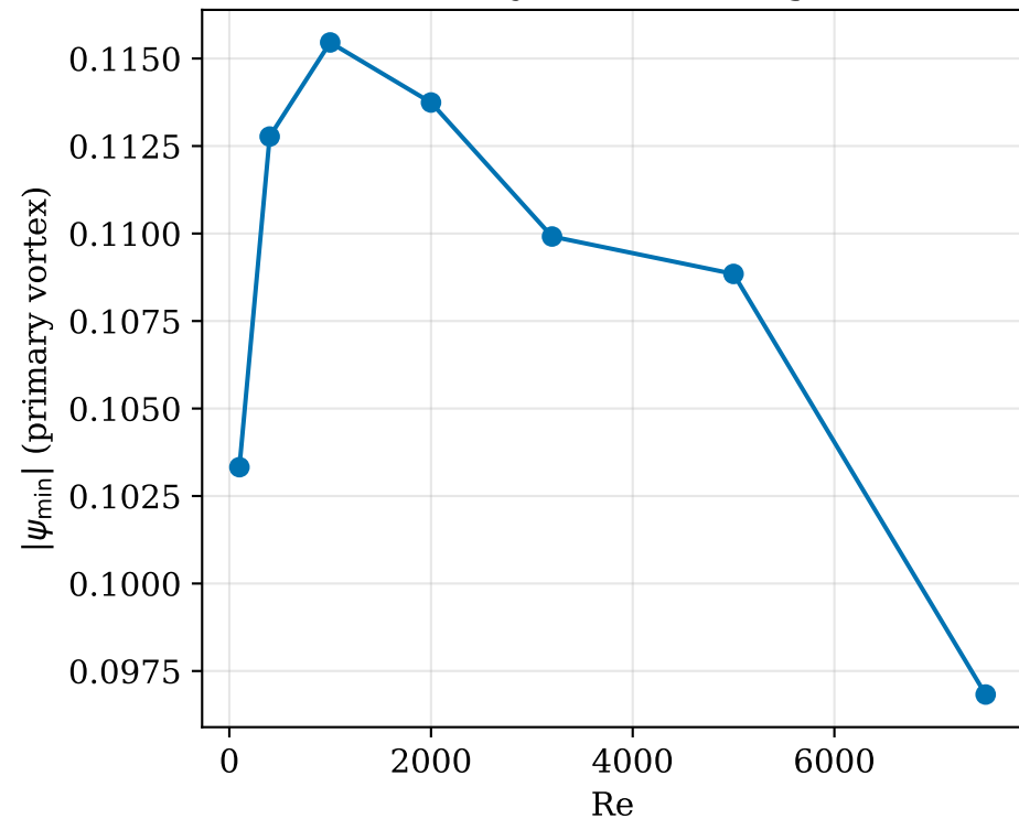
Primary-vortex strength
