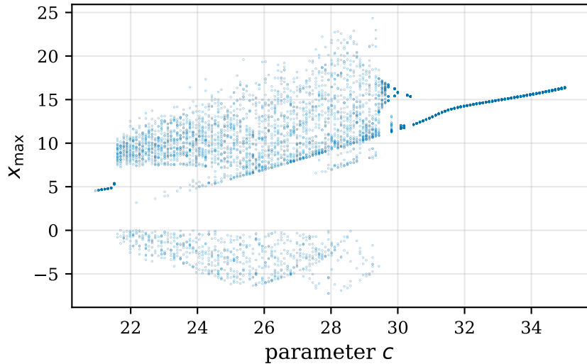
(a) Bifurcation vs c ( q = 0.95 )
