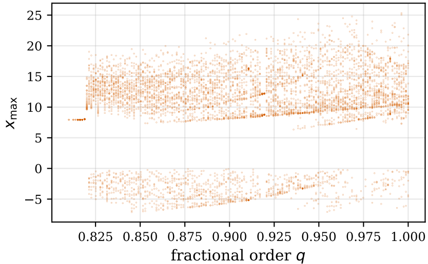
(b) Bifurcation vs q ( c = 28 )
