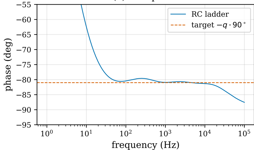
(b) FOC phase
