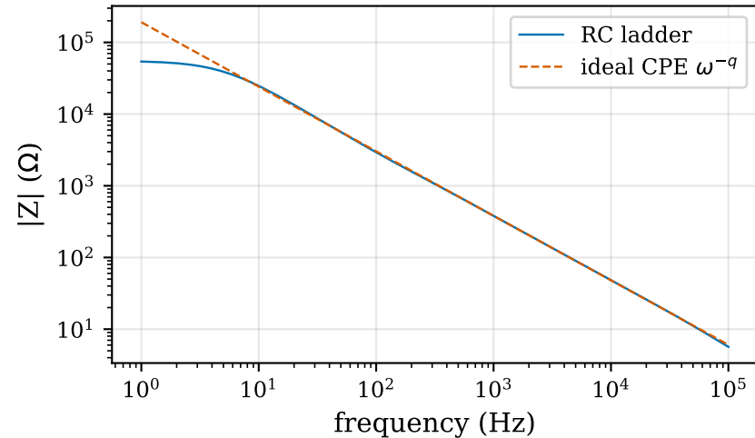
(a) FOC magnitude
