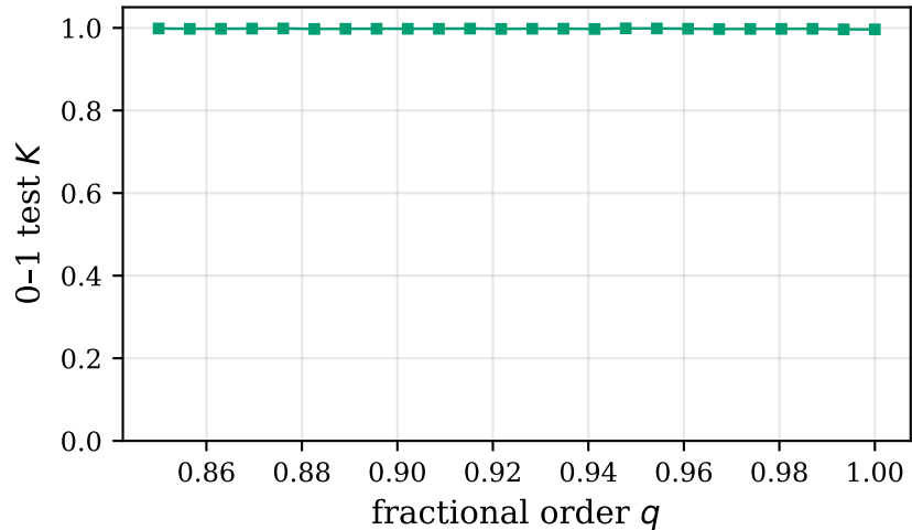
(b) 0-1 test for chaos
