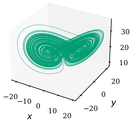
(c) 3D attractor
