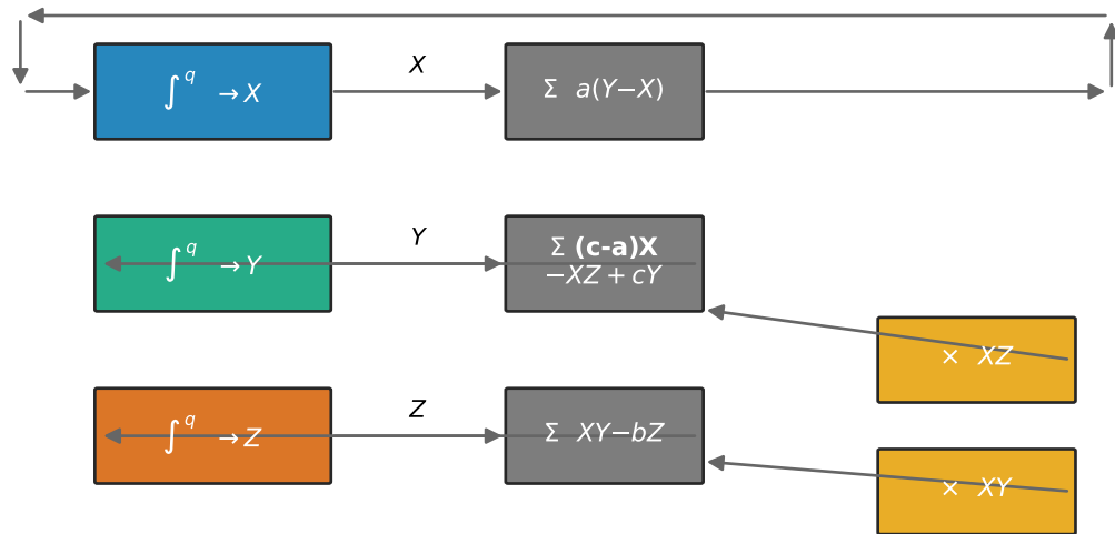
(a) Analog signal-flow realisation
