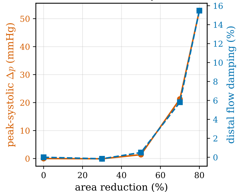
(a) Stenosis severity effect
