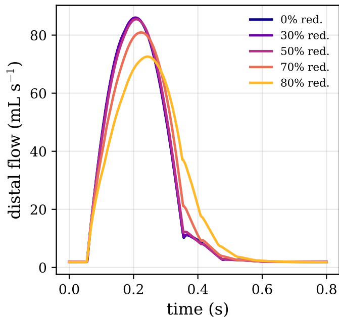
(b) Distal flow waveforms
