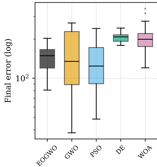
F5 Rastrigin
