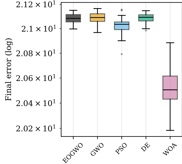
F8 Ackley
