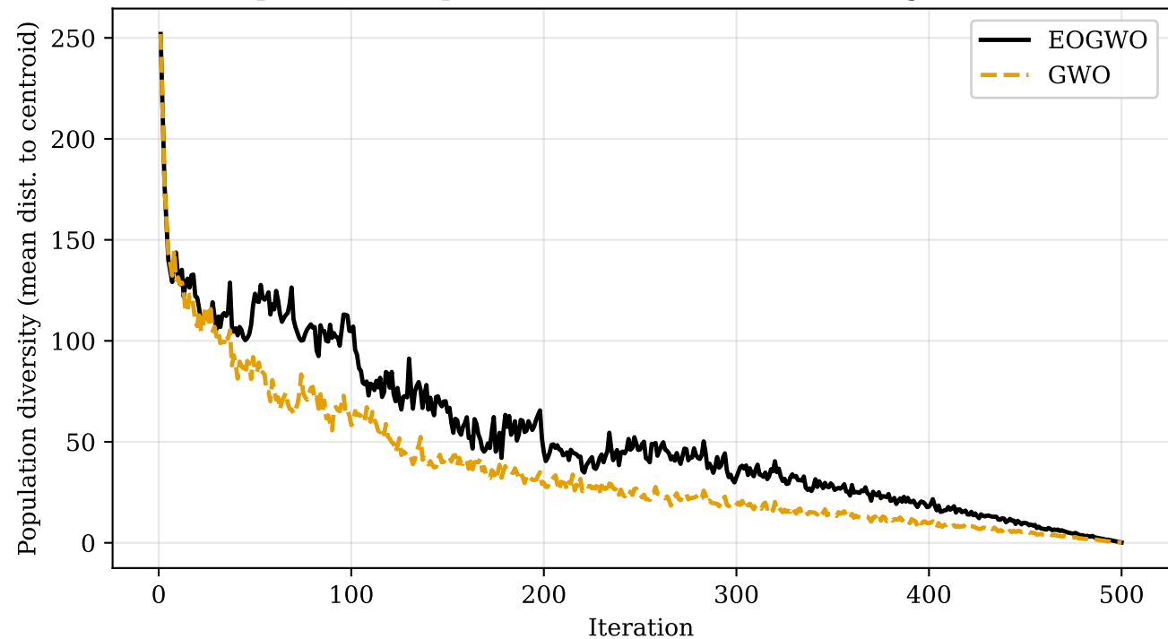
Exploration--exploitation balance on F5 (Rastrigin, D=30)
