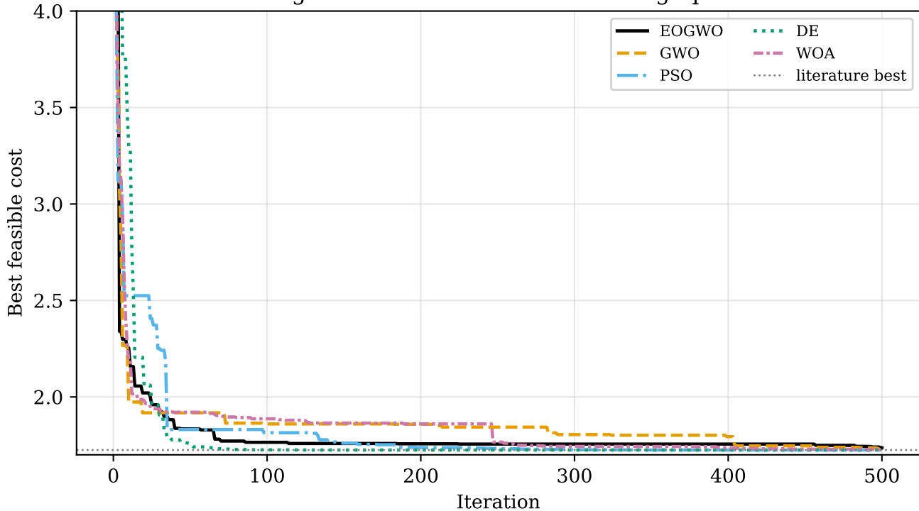
Convergence on the welded-beam design problem
