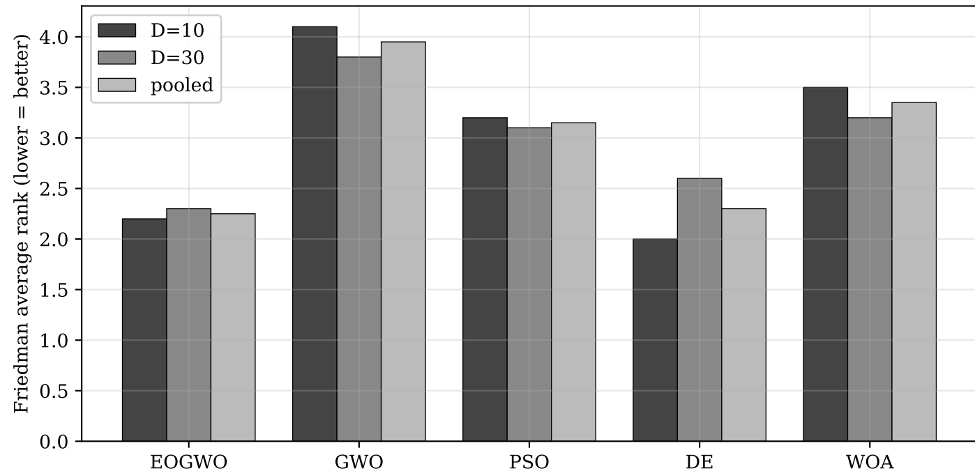
Friedman average ranks across benchmark functions
