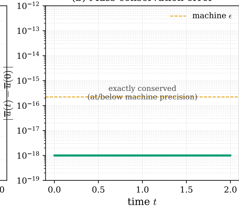
(b) Mass-conservation error
