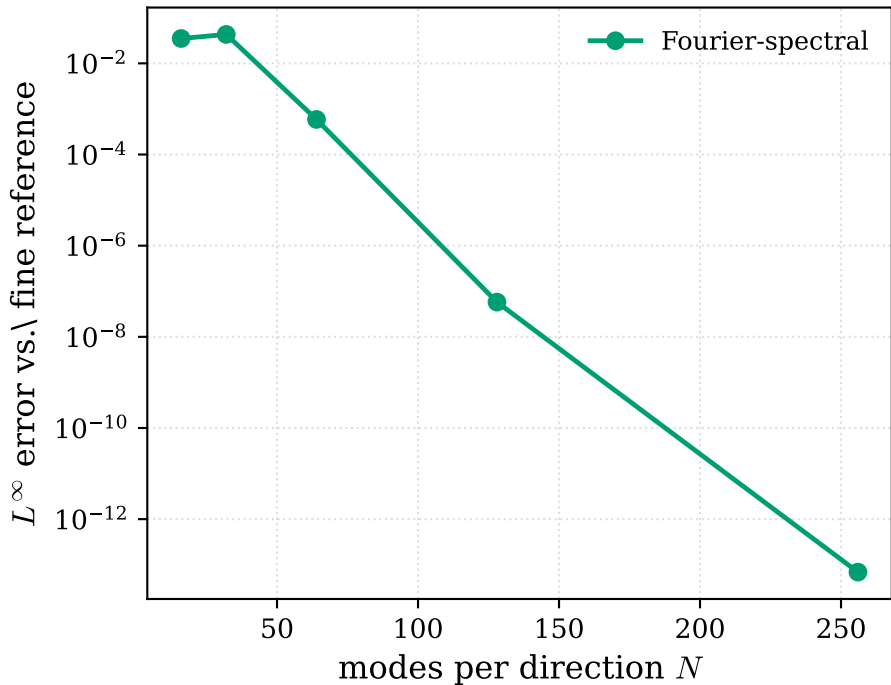
Spatial spectral convergence (1D)
