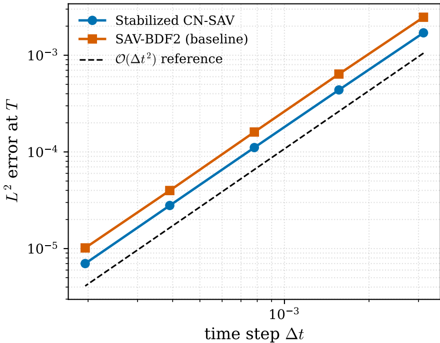
Temporal convergence (1D Cahn--Hilliard)
