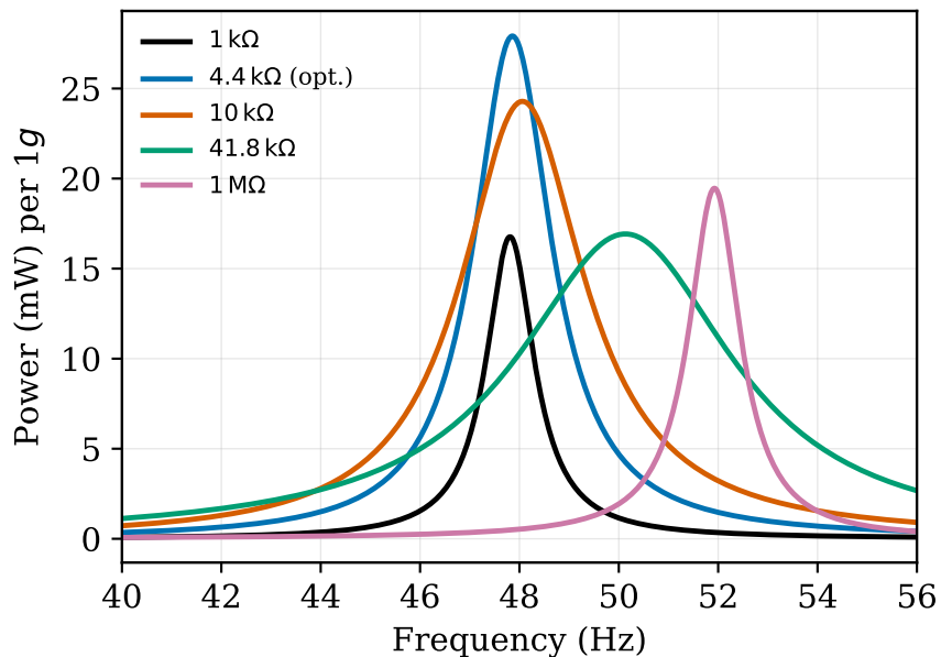
(b) Power FRF
