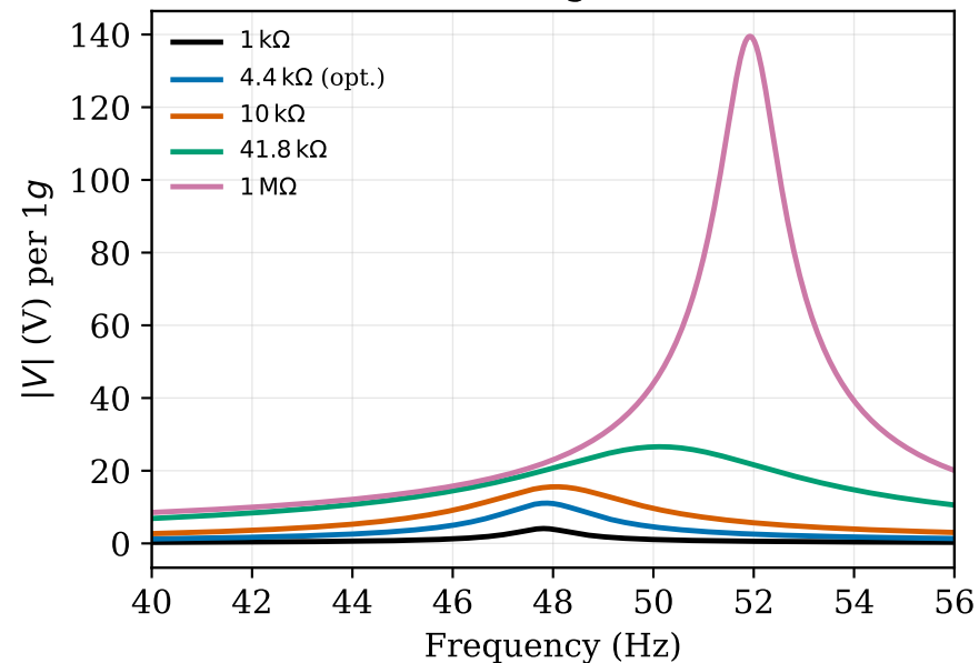
(a) Voltage FRF
