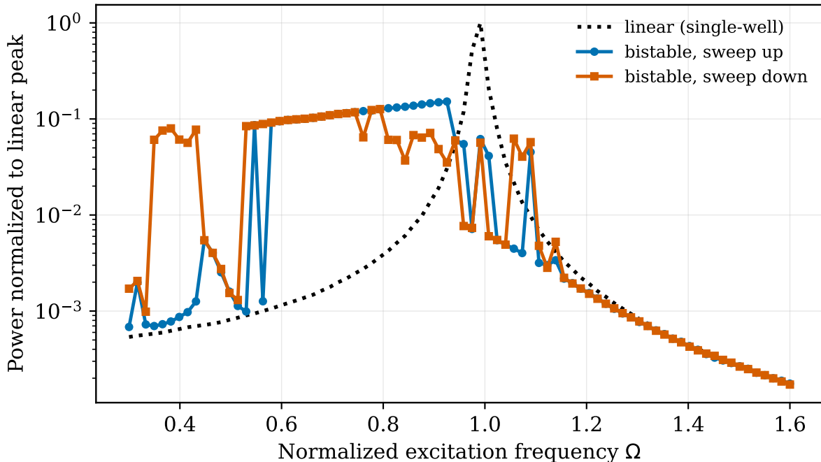
Broadband snap-through orbit vs linear resonance
