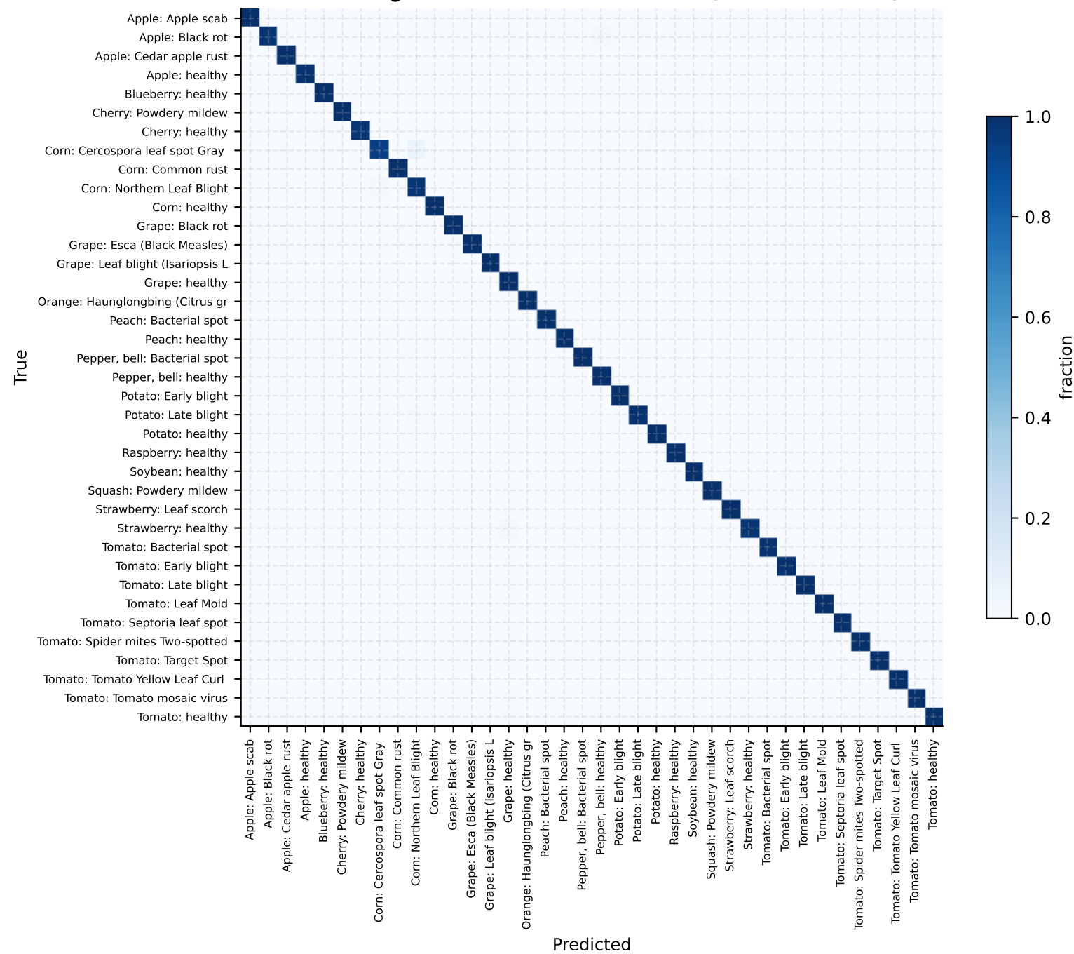
PlantVillage test-set confusion matrix (row-normalised)
