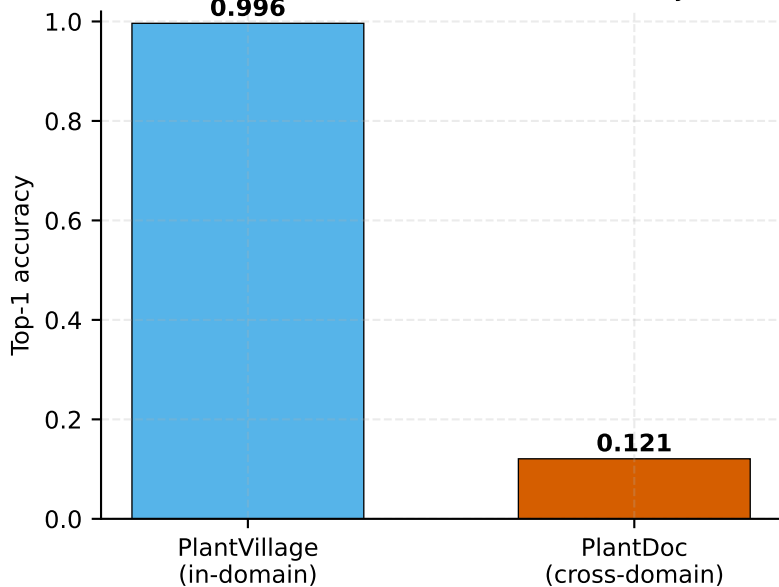
In-domain vs. cross-domain accuracy
