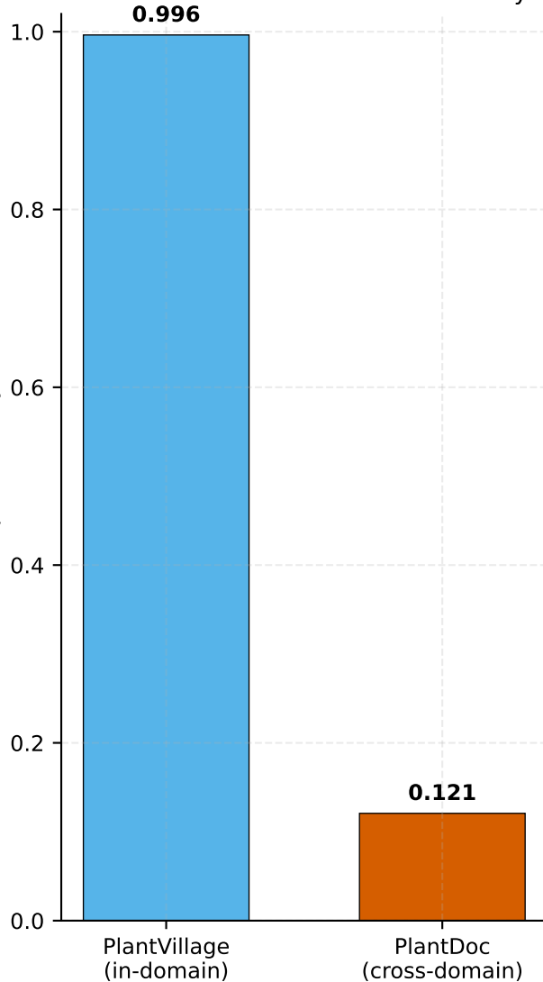
In-domain vs. cross-domain accuracy
