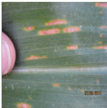
PlantDoc: Corn
