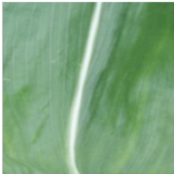
PlantDoc: Corn
