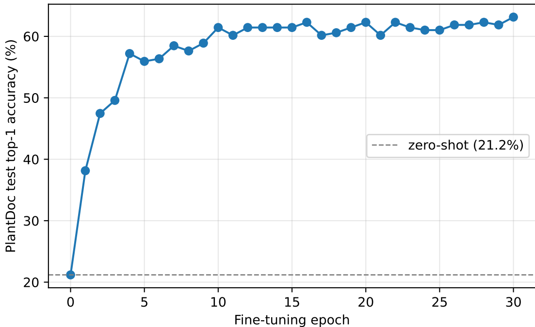
Target-domain fine-tuning on PlantDoc
