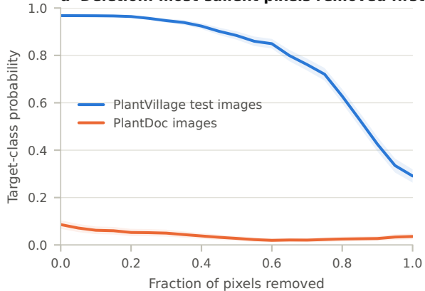
a Deletion: most-salient pixels removed first
