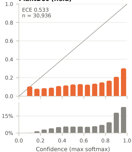
PlantDoc (field)
