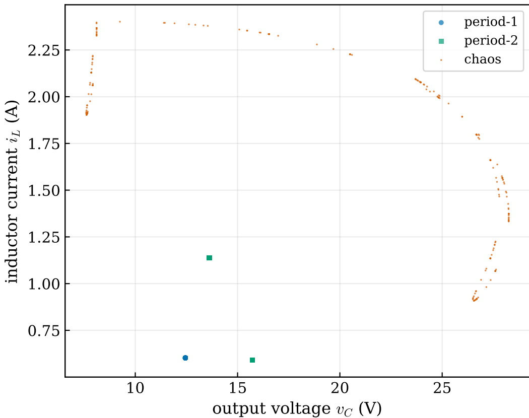
Poincaré section (sampled at clock instants)
