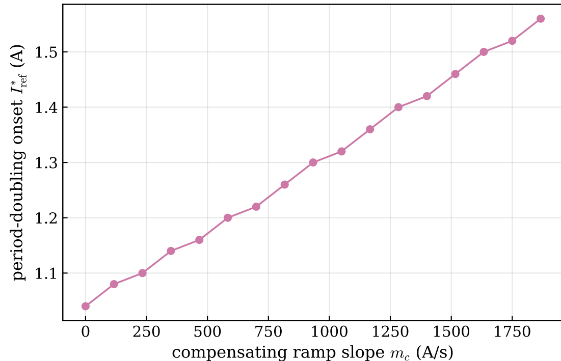
Stable-operation boundary vs slope compensation
