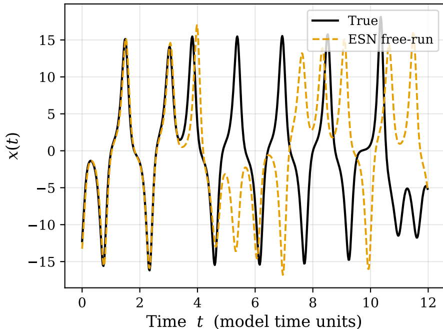
(b) Autonomous prediction of x -coordinate
