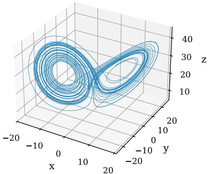
(a) Lorenz attractor (ground truth)
