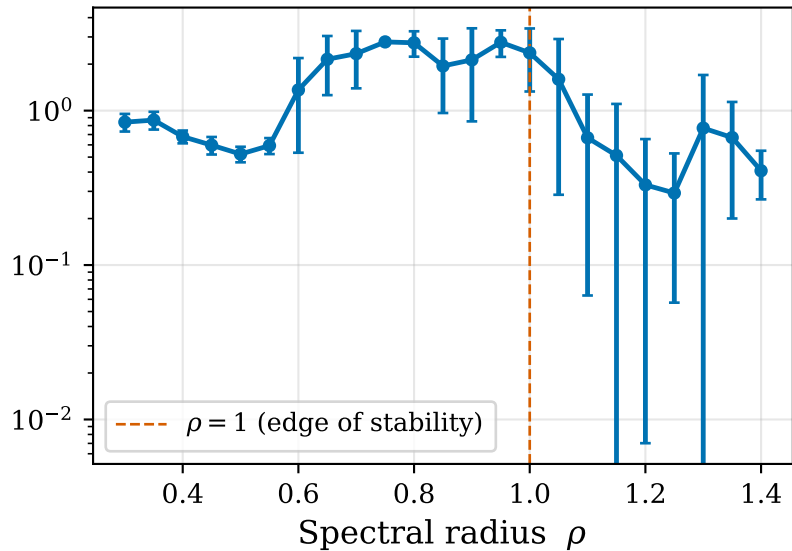
NRMSE (1 Lyapunov time)
