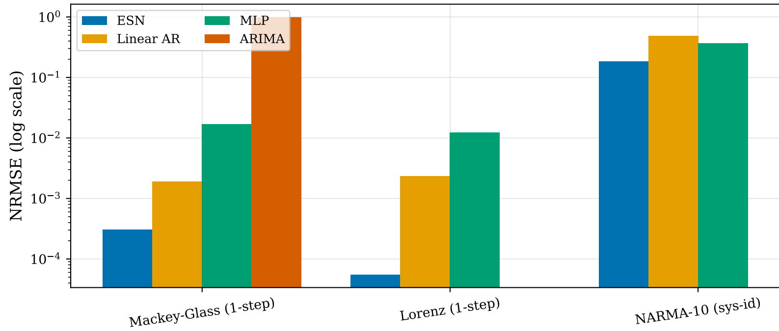
ESN vs. baselines across benchmark tasks
