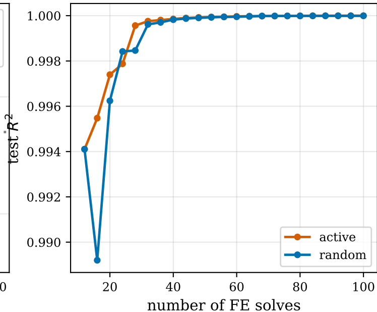
Test R^2 vs budget
