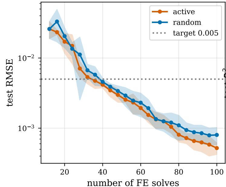
Active vs random sampling
