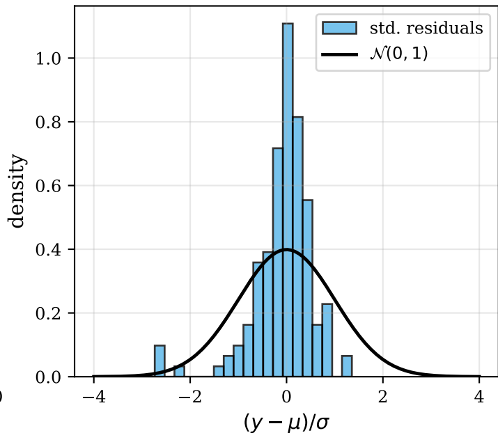
Standardized residuals
