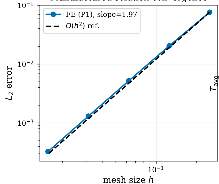
Manufactured-solution convergence
