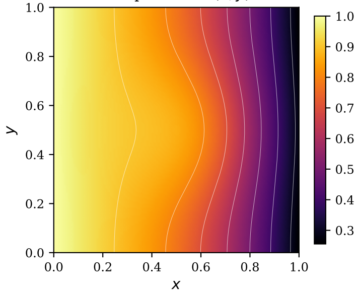
Temperature u(x, y)
