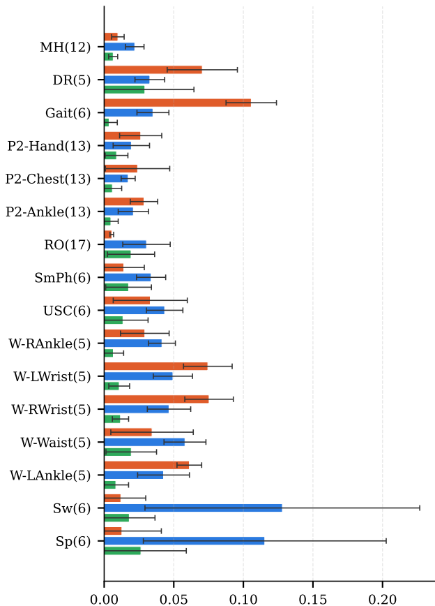
Mean MDI per feature (catch: top-15 | score/original: all)
