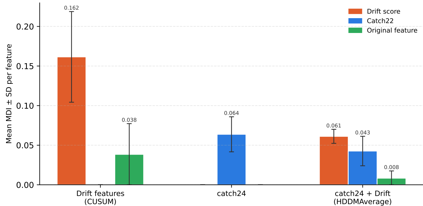
Informative efficiency by feature type (MDI — RF) — W-LAnkle (catch: top-5; score/original: all)
