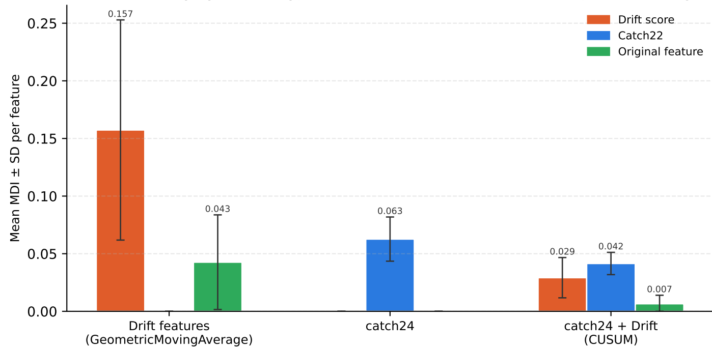
Informative efficiency by feature type (MDI — RF) — W-RAnkle (catch: top-5; score/original: all)
