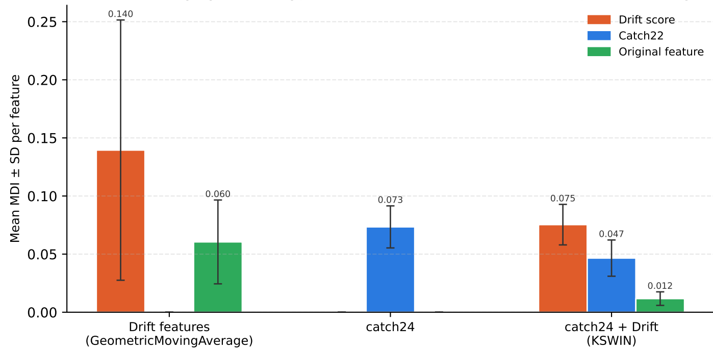
Informative efficiency by feature type (MDI — RF) — W-RWrist (catch: top-5; score/original: all)
