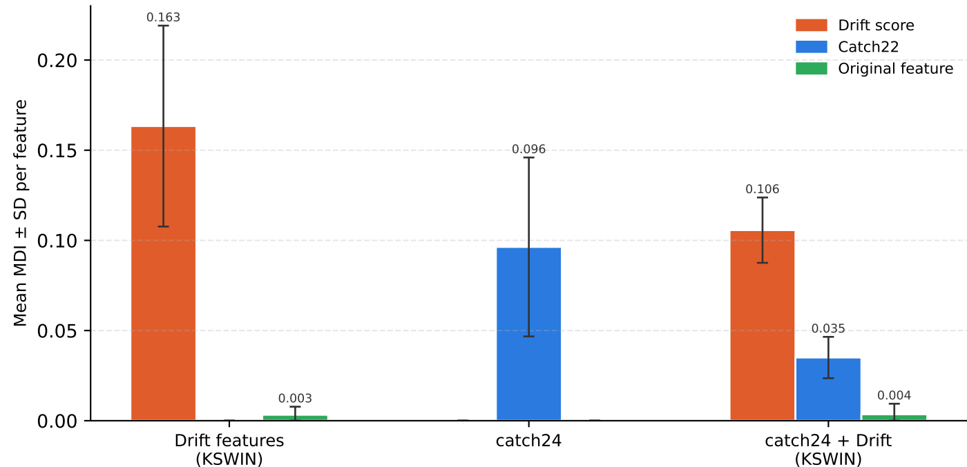
Informative efficiency by feature type (MDI — RF) — gait (catch: top-6; score/original: all)
