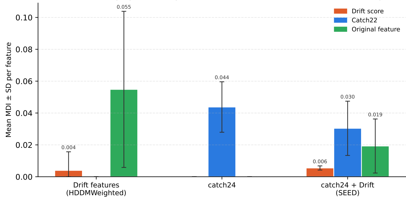
Informative efficiency by feature type (MDI — RF) — occ (catch: top-17; score/original: all)
