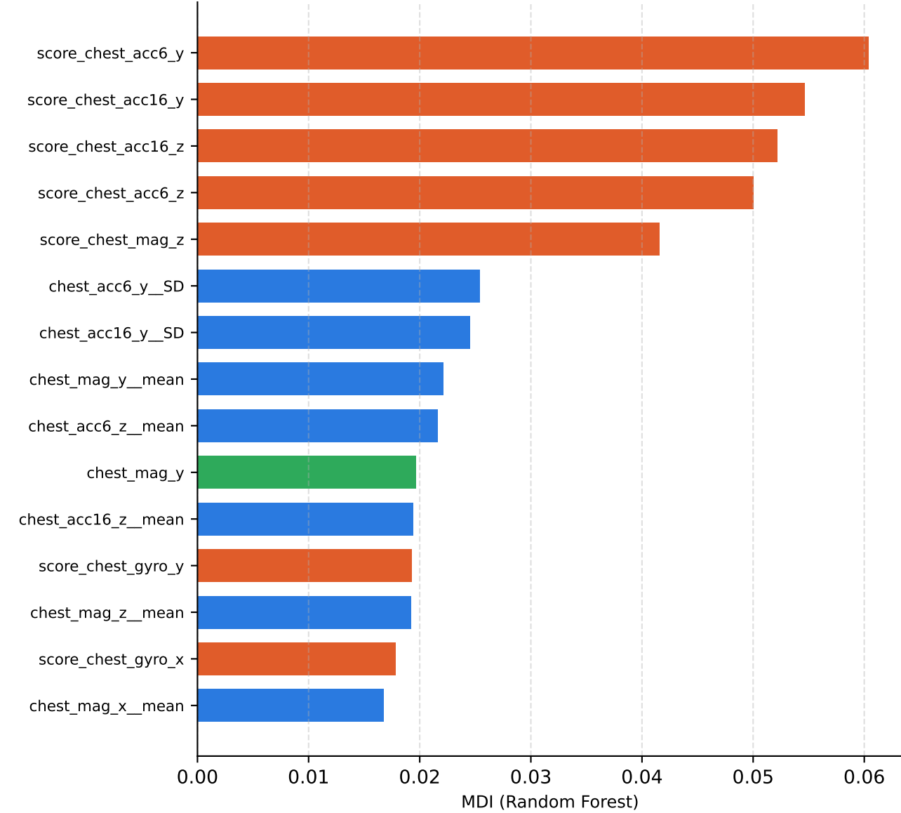
C3 — catch24 + Drift (GeometricMovingAverage)
