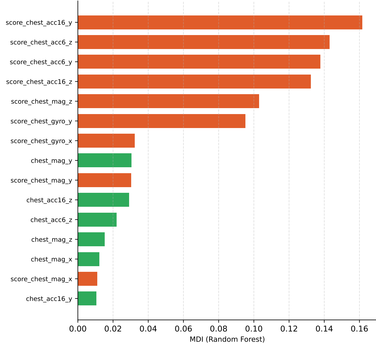
C1 — Drift features (GeometricMovingAverage)
