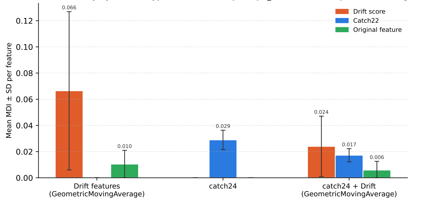
Informative efficiency by feature type (MDI — RF) — pamap2_chest (catch: top-13; score/original: all)
