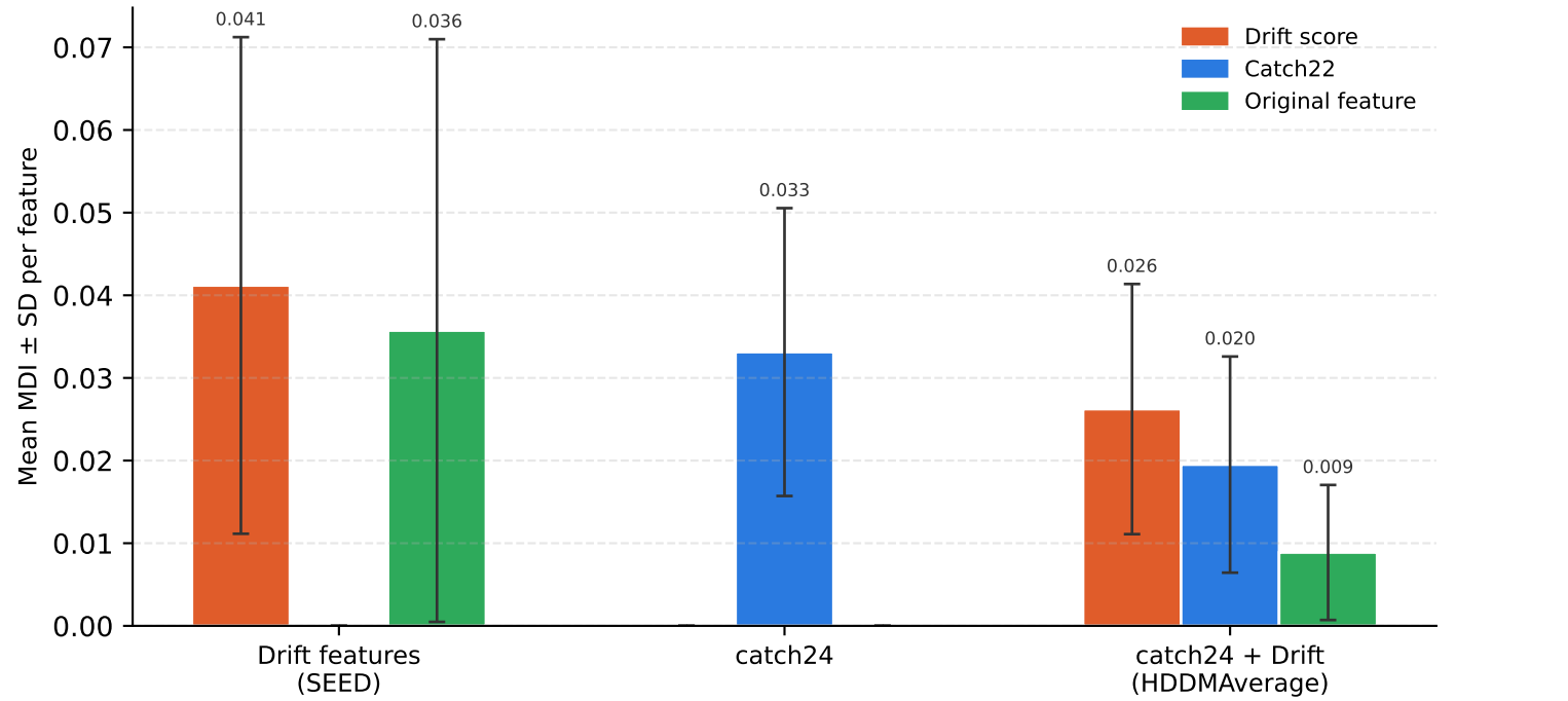
Informative efficiency by feature type (MDI — RF) — pamap2_hand (catch: top-13; score/original: all)
