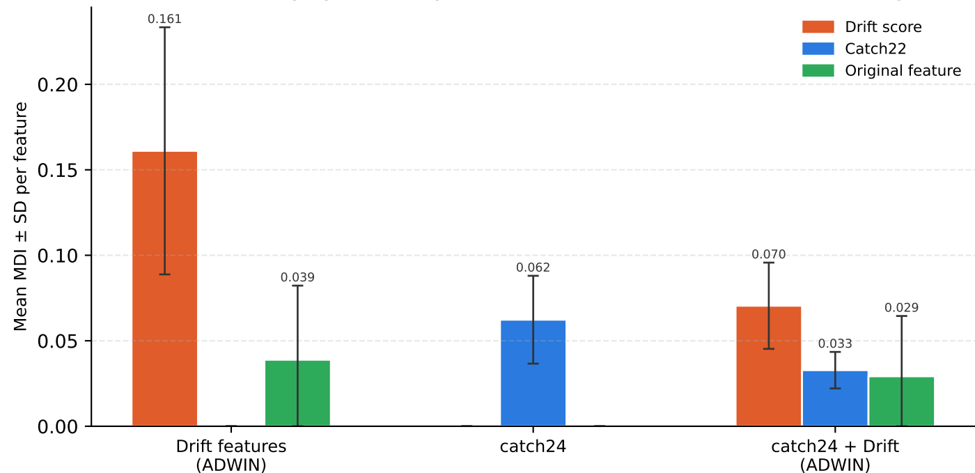
Informative efficiency by feature type (MDI — RF) — rs (catch: top-5; score/original: all)
