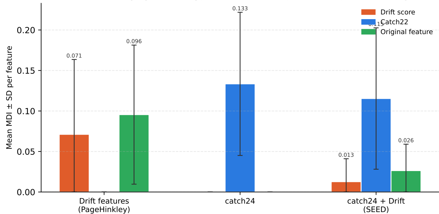
Informative efficiency by feature type (MDI — RF) — sp (catch: top-6; score/original: all)
