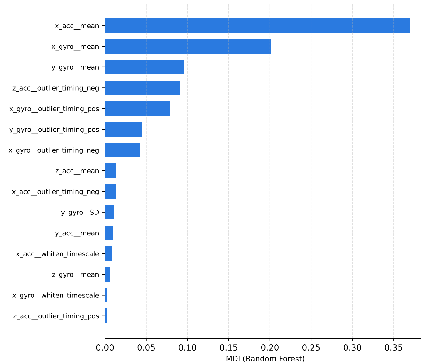
C2 — catch24
