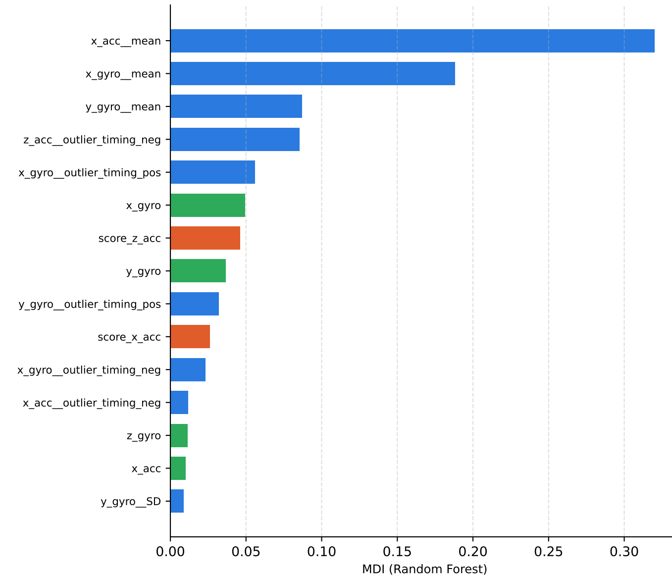
C3 — catch24 + Drift (GeometricMovingAverage)
