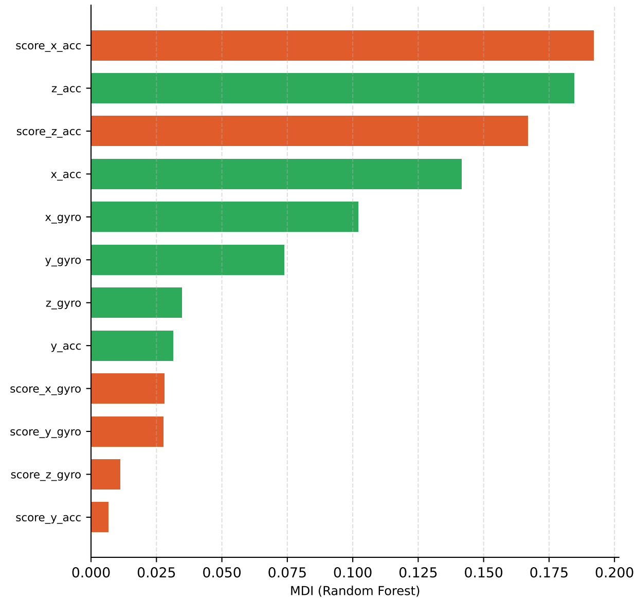
C1 — Drift features (CUSUM)
