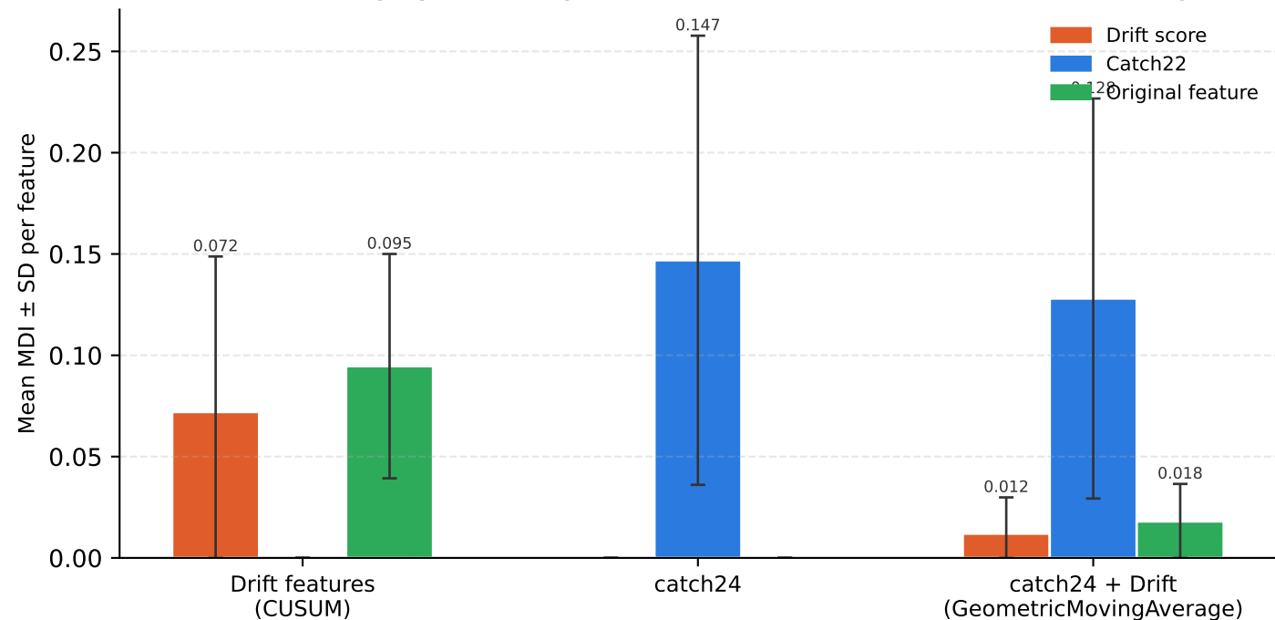
Informative efficiency by feature type (MDI — RF) — sw (catch: top-6; score/original: all)
