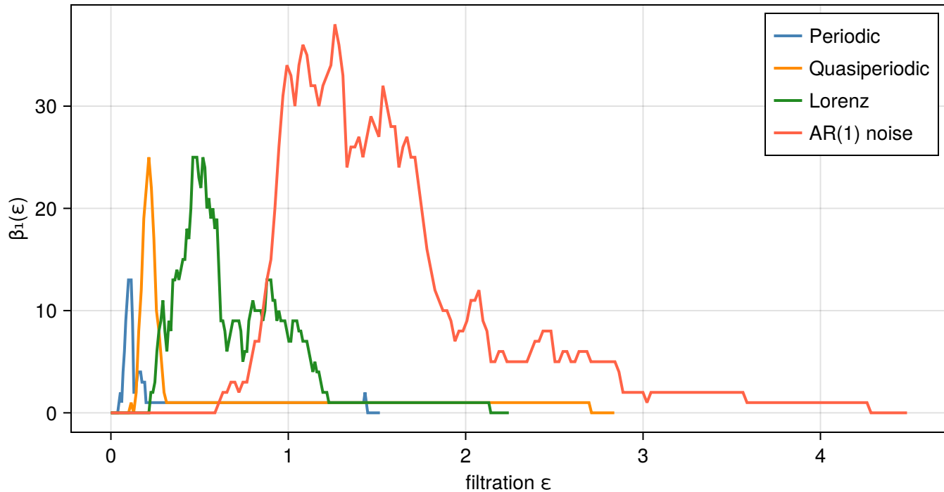
H 1 Betti Curves
