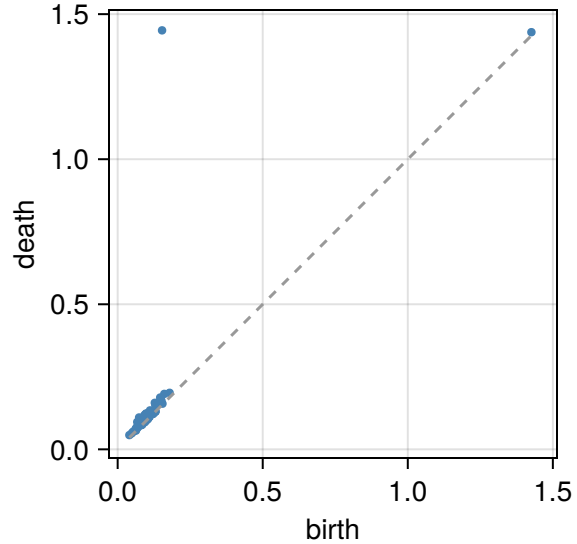
H 1 — Periodic
