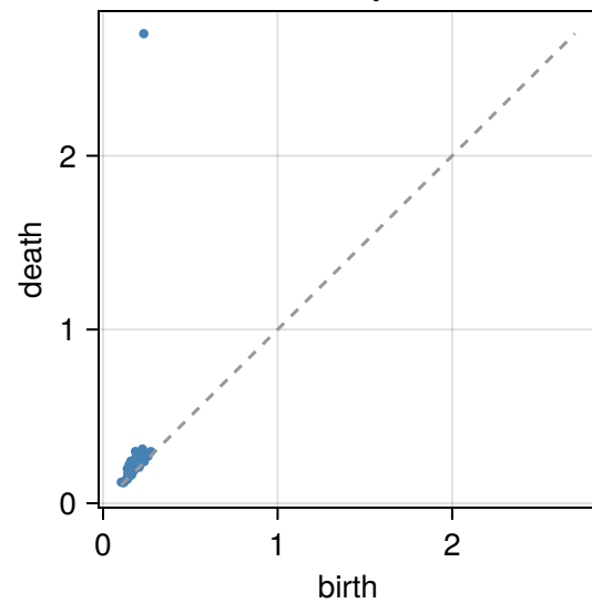
H 1 — Quasiperiodic
