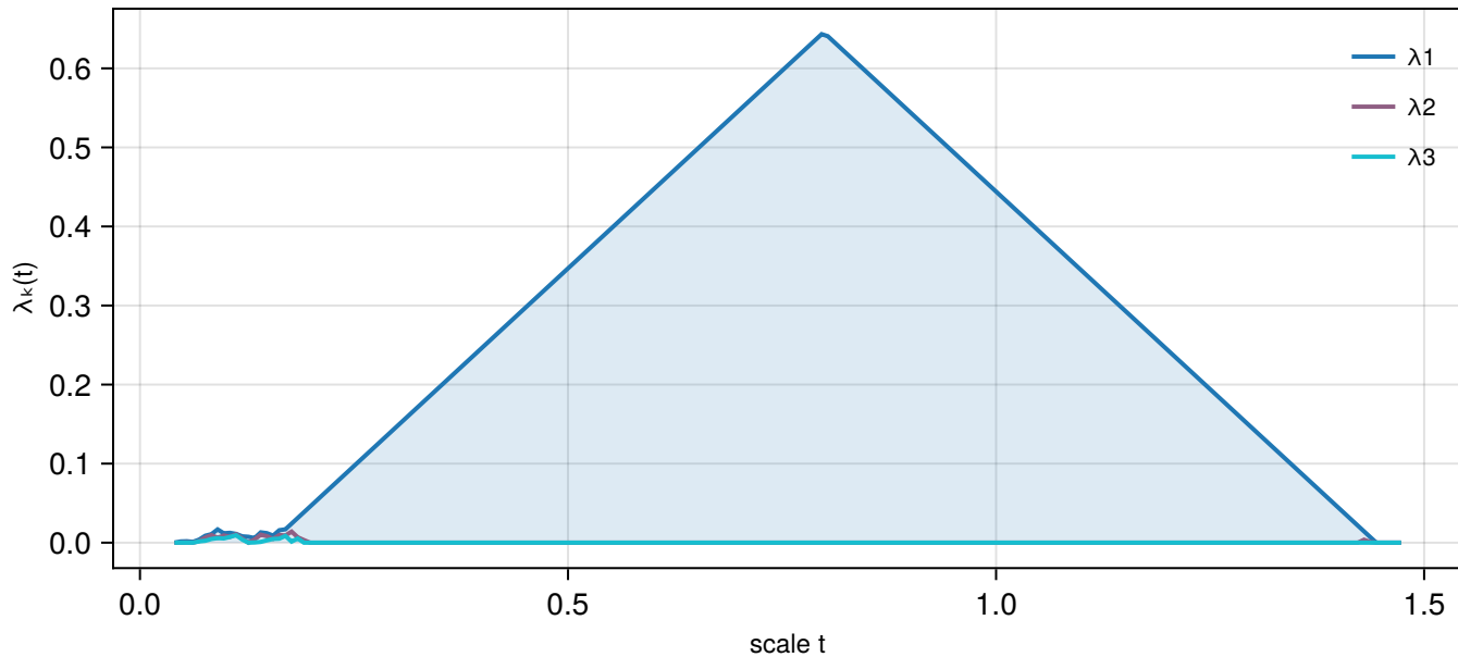
H 1 Persistence Landscape — periodic (3 layers)
