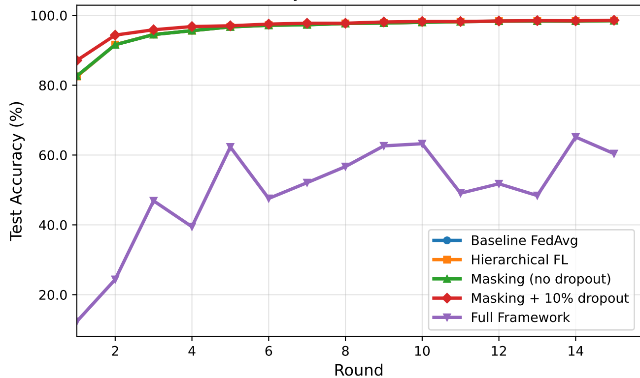
Test Accuracy vs. Communication Round
