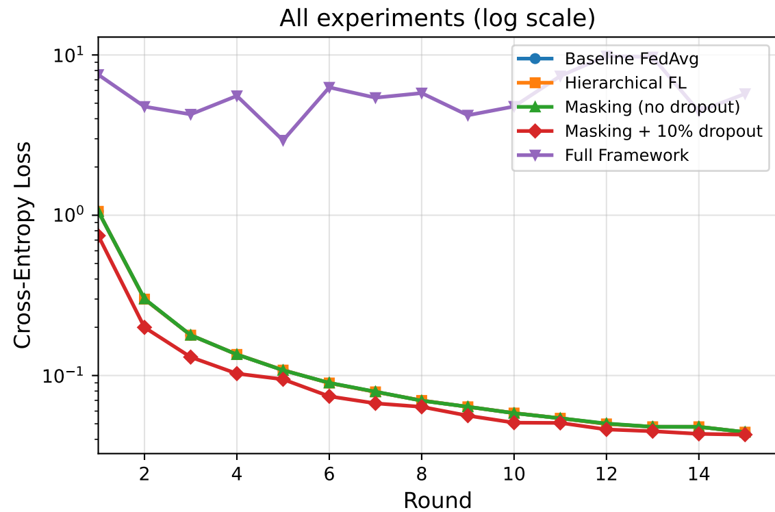
Test Loss vs. Communication Round
